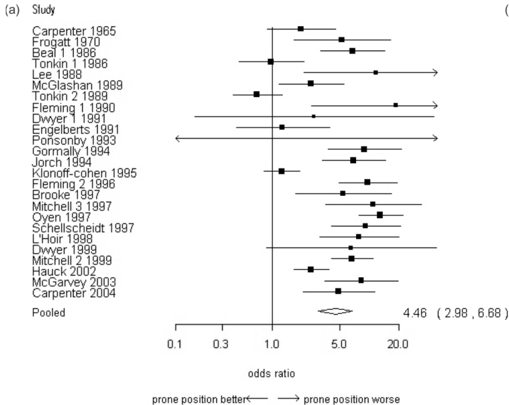
meta-analysis
