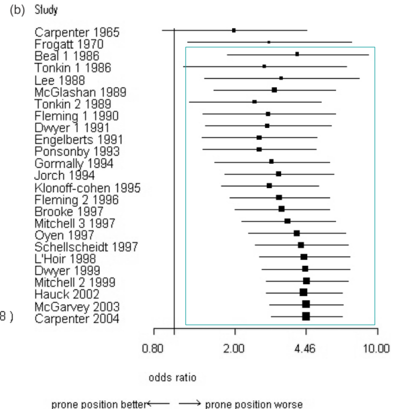
cumulative meta-analysis
